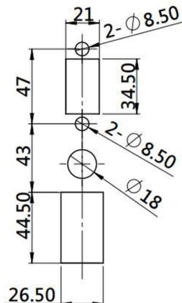
PANEL CUTOUT MS460-1-1G
